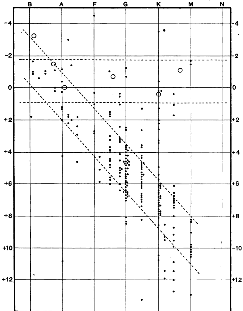
FIG. 19.—Absolute Magnitudes of Stars (Russell).
